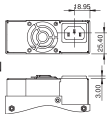
FAN+IEC OPTION
