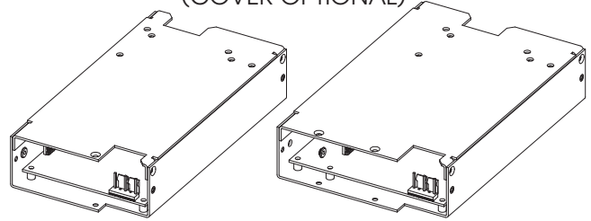
'U' CHASSIS (COVER OPTIONAL)
